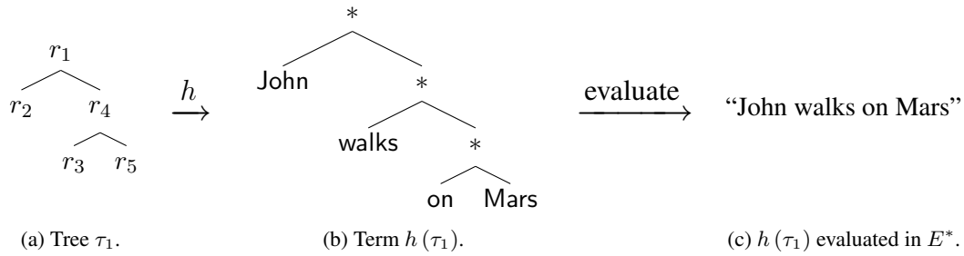
Figure 2: The tree \tau_1 , evaluated by the homomorphism h and the algebra E^*
