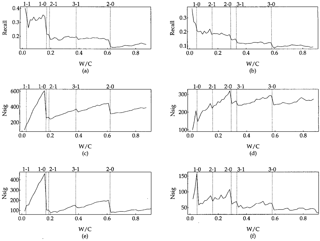
Figure 3 Results of word extraction procedure ( \alpha = 0.05 ) with A-B distributions. Panels (a), log-likelihood ratio, G^2 , and (b), Fisher’s exact test, show the recall results of the extraction procedure for corpus 2. Panels (c) and (d) show the total number of significant words ( N_{sig} ), again for G^2 and Fisher’s exact test, respectively (see also Figure 2). Panels (e) and (f) show the results for a randomized corpus for G^2 and Fisher’s exact test. The numbers above the panels indicate the A-B distribution of the contingency tables in Table 2.
