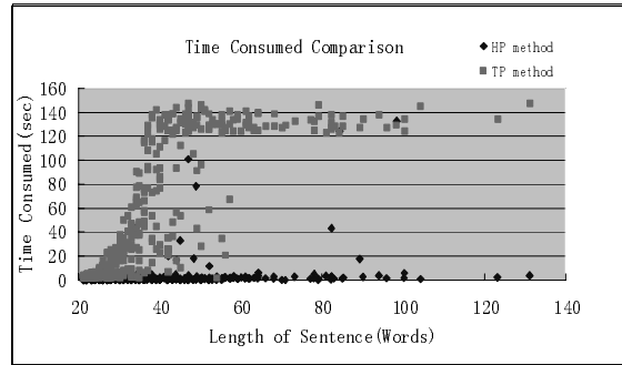
Figure 5. Time consumption
