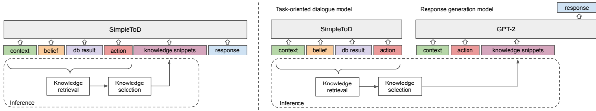
Figure 4: Illustration of the models. Left : the SimpleToDPlus model; Right : the Combiner model;
