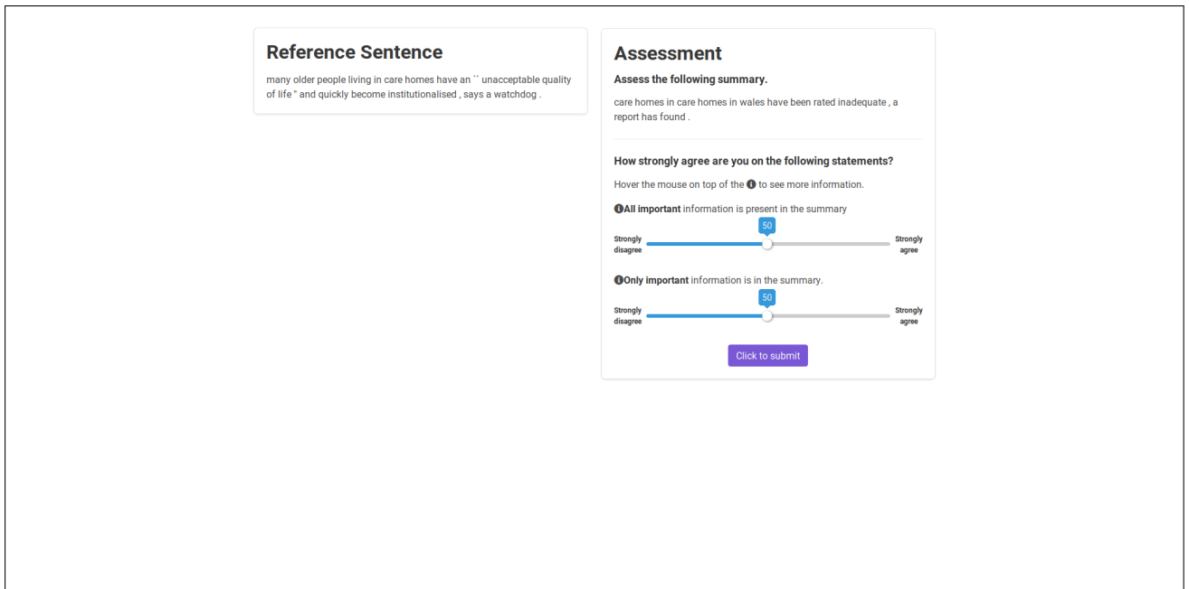
Figure 5: The UI for content evaluation using reference summary as comparison. At the right of the page judges give the recall and precision assessment by sliding the scroller from 1 to 100 based on the given summary quality.
