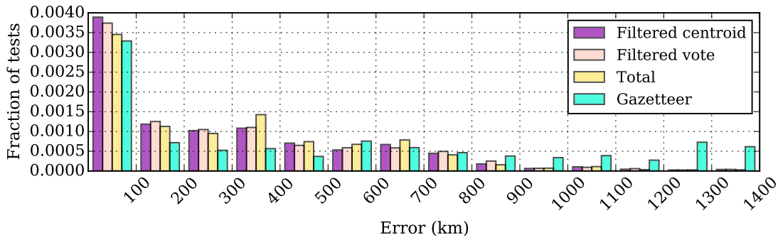
Figure 7: Comparing models with placeness threshold at \log T = 20 .
