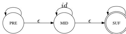
Figure 4: Clitic concatenation
