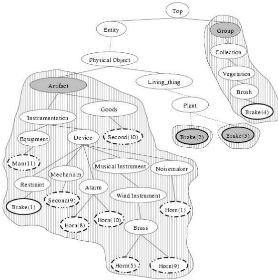
Figure 1: Subhierarchies resulting from the disambiguation of brake with the context words \{horn, man, second\} . Example extracted from the Senseval-3 english-all-words test corpus. ( M_1 = 11 , nh_1 = 21 , M_2 = M_3 = nh_2 = nh_3 = 1 , M_4 = 1 , nh_4 = 5 , where M_i and nh_i indicates, respectively, the M and nh values for the i -th sense)
