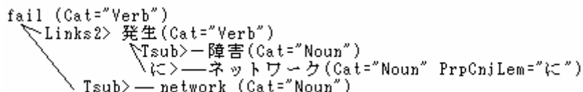
Fig. 4. Part of the Mindnet Entry for “fail”
