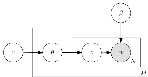
Figure 1: Graphical Model for LDA
