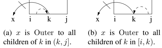
Figure 10: The edge \vec{e}_{kx} is guaranteed to be crossed, so k is in a BadContext for whichever side it does not get its parent from.
