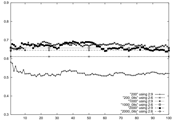
Figure 2: F for NE over iterations, baselines
