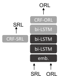
Figure 2: Hierarchical-MTL (H-MTL).
