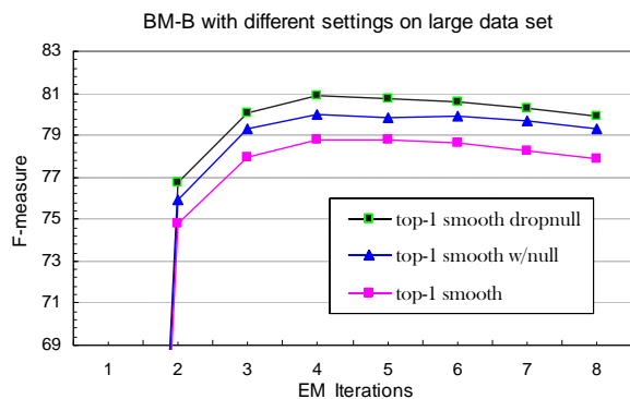
Figure 6: BM-B with different settings on large data
