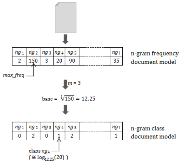
Figure 1. Steps for computing the n-gram classes of a document. The number of classes in this example is 3 (class labels are from 0 to 2).
