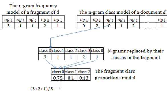
Figure 2. Steps for representing a document fragment by the proportion of 3 n-gram classes.
