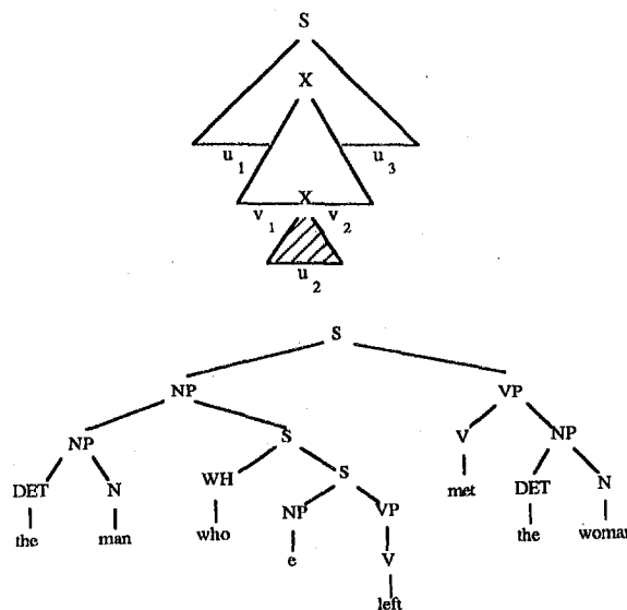
Figure 3: The operation of adjoining
