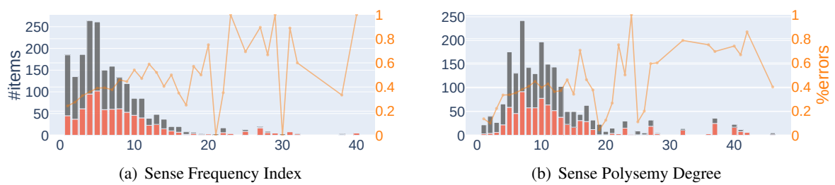
Figure 5: Evaluation on DeepL
