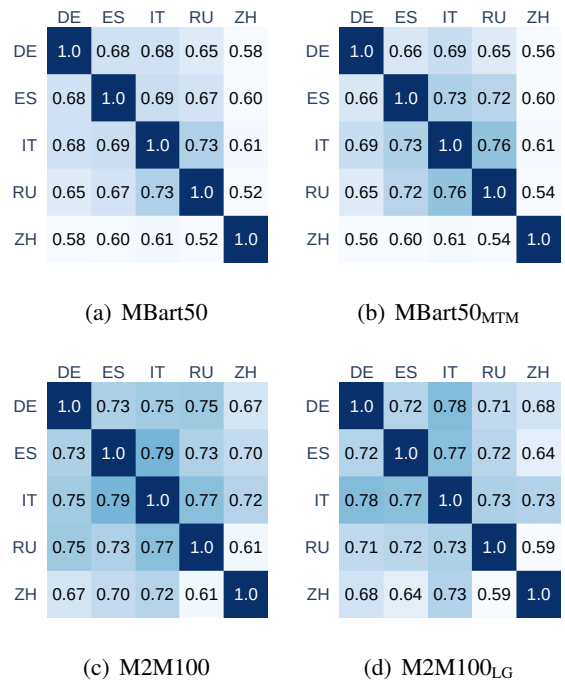
Figure 4: Language Frequency Correlation: percentage of times that an item translates to the same synset.
