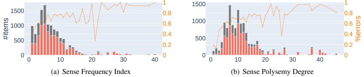
Figure 3: Overall distribution of errors, summed across all models and languages, with respect to (a) Sense Frequency Index ( \mu_{\lambda_P}(\sigma) ) and (b) Sense Polysemy Degree ( \delta_{EN}(\lambda_P) ). Red bars represent the number of errors (i.e., BAD items) for a given group, grey bars represent the number of correct (i.e., GOOD items) items. Orange lines represent the percentage of errors (i.e., \frac{\#BAD}{\#GOOD+\#BAD} ) for a given group.
