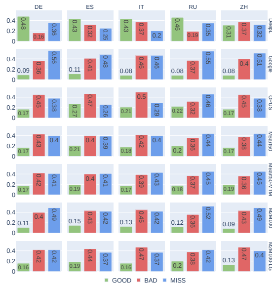
Figure 2: General results of the analysis. Numbers represent percentages of the whole dataset (600 items). A full-page version of this image, for readability purposes, is available in the Appendix (Figure 16).
