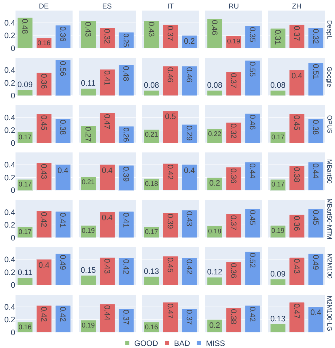
Figure 16: Full page version of Figure 2.
