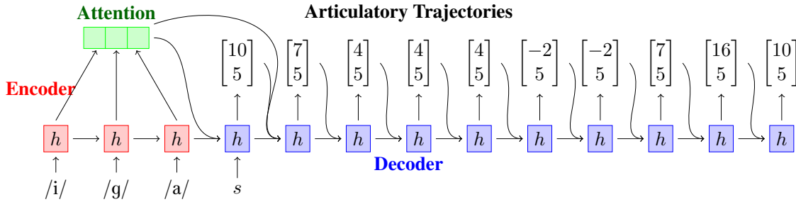
Figure 8: Sequence-to-sequence recurrent neural network with encoder-decoder attention. For sample input /ig-a/, the model outputs at each timepoint a two-dimensional vector containing predicted values for tongue body and lip constriction degrees. While attention is shown as part of the input only to the first two decoder hidden states, it is part of the input for all hidden states in our models.
