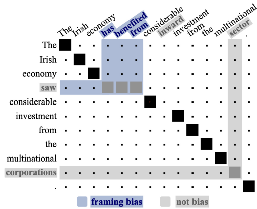
Figure 1: Word Alignment and Bias Annotation example for a pre-edited (top) and post-edited (left) sentence pair. Grey block ■ means non-identical word/phrases alignment. Three edits are extracted: has benefited from → saw , inward → [NULL] (Deletion), sector → corporations while the first is labelled as framing bias .
