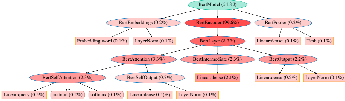
Figure 5: Abridged view of a BERT-base-uncased model annotated with predicted energy from our prediction method. The root contains the absolute energy of the model while every other node is annotated with its respective energy percentage share. Darker colors represent nodes that consume a higher percentage of energy. There are 12 BertLayer modules in the actual model. We show just one for brevity. The shown energy is an average of energy of the node across all (batch size, sequence length) models of BERT-base-uncased type.
