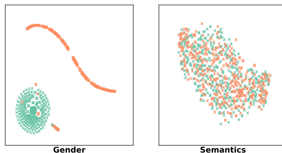
Figure 2: A visualization of the disentangled features using t-SNE plot. Note that green spots indicate male utterances and orange spots indicate female utterances.
