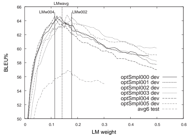
Figure 3: Sections along the LM weight axis of score functions of six different optimizer samples and of the avg6 system.
