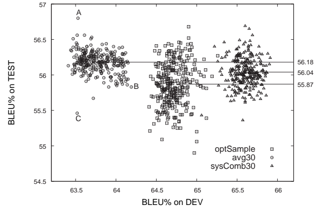
Figure 2: Scatter plots of optSample , avg30 and sysComb30 for the ar-en BTEC task.
