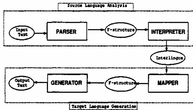
Figure 2: Four Major KANT Modules
