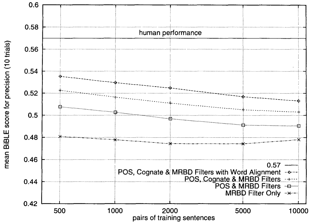
Figure 5: The large MRBD resulted in the most useful filter for this pair of languages. The scores for the cascade of all the filters (the highest curve) are close to the human performance of 0.57.
