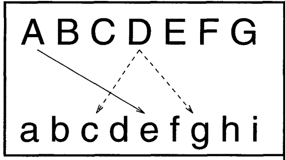
Figure 4: One of the heuristics used in the Word Alignment Filter — Crossing partitions are minimized by aligning D with g rather than with c.
