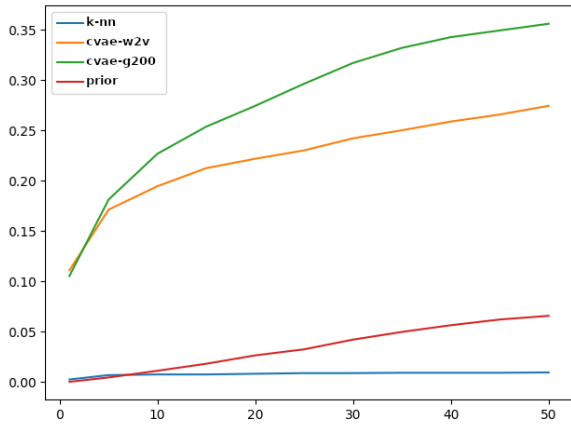
Figure 2: Computed accuracy for the different models. The X axis shows different percentages of retained out-predictions, starting from the most probable ones (parameter L). The Y axis shows the obtained accuracy.
