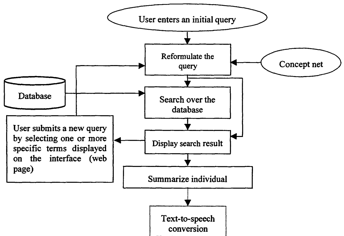
Fig. 2 System Data Flow
