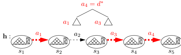
Figure 6: An example history of states and actions, where actions that are part of the reference derivation d^* = a_4 are in red. The compressed history is c(\mathbf{h}) = (s_1, a_1, s_3, a_3, s_4, a_4, s_5) .
