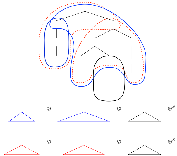
Figure 4: Above: an example of a set of fragments extracted from the tree in Figure 1. Below: two incremental derivations that generate it. Colors (and lines strokes) indicate which derivation fragments belong to.
