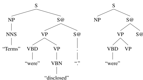
Figure 1: An example of a binarized 2 parse tree and a lexicalized fragment extracted from it.
