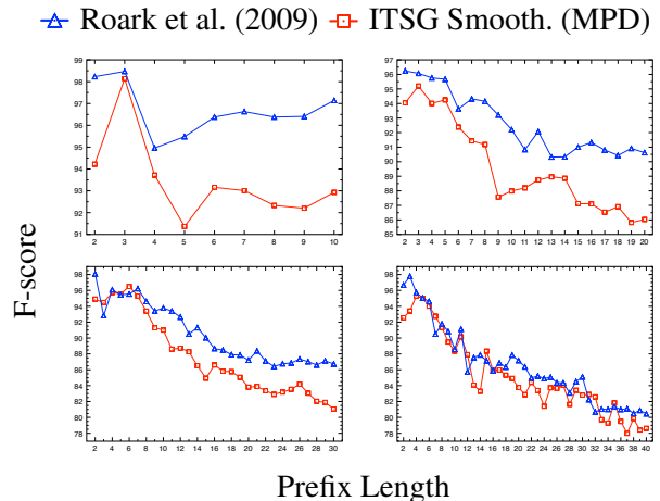
Figure 8: Partial parsing results for sentences of length 10, 20, 30, and 40 (from upper left to lower right).
