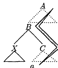
Figure 2: The highly distinctive ‘zig-zag’ or ‘lightning bolt’ configuration of nodes in the analysis tree characteristic of the use of production schema (4.f) in transform \mathcal{LC}_4 . This is the only configuration which causes an increase in stack depth in a top-down parser using a grammar transformed with \mathcal{LC}_4 .
