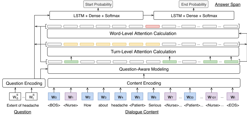
Figure 1: Turn-based hierarchical architecture for dialogue comprehension: tokens in purple are the indicators of dialogue turns, and their indices are used to select question-aware hidden states (Green) for turn-level attention calculation. The turn with higher attentive score (Yellow) contributes more in scoring word-level attentions (Red).
