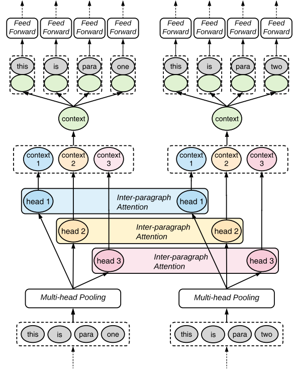
Figure 2: A global transformer layer. Different colors indicate different heads in multi-head pooling and inter-paragraph attention.
