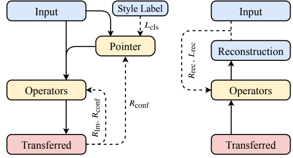
Figure 2: Graphical overview for the training algorithm, which consists of a transfer step (left) and a reconstruction step (right). Solid lines denote forward pass; dotted lines denote rewards or losses. Blue / red items belong to the source / target styles; yellow items denotes the agents. Best viewed in color.
