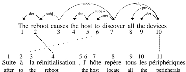
Figure 1: A cohesion constraint violation
