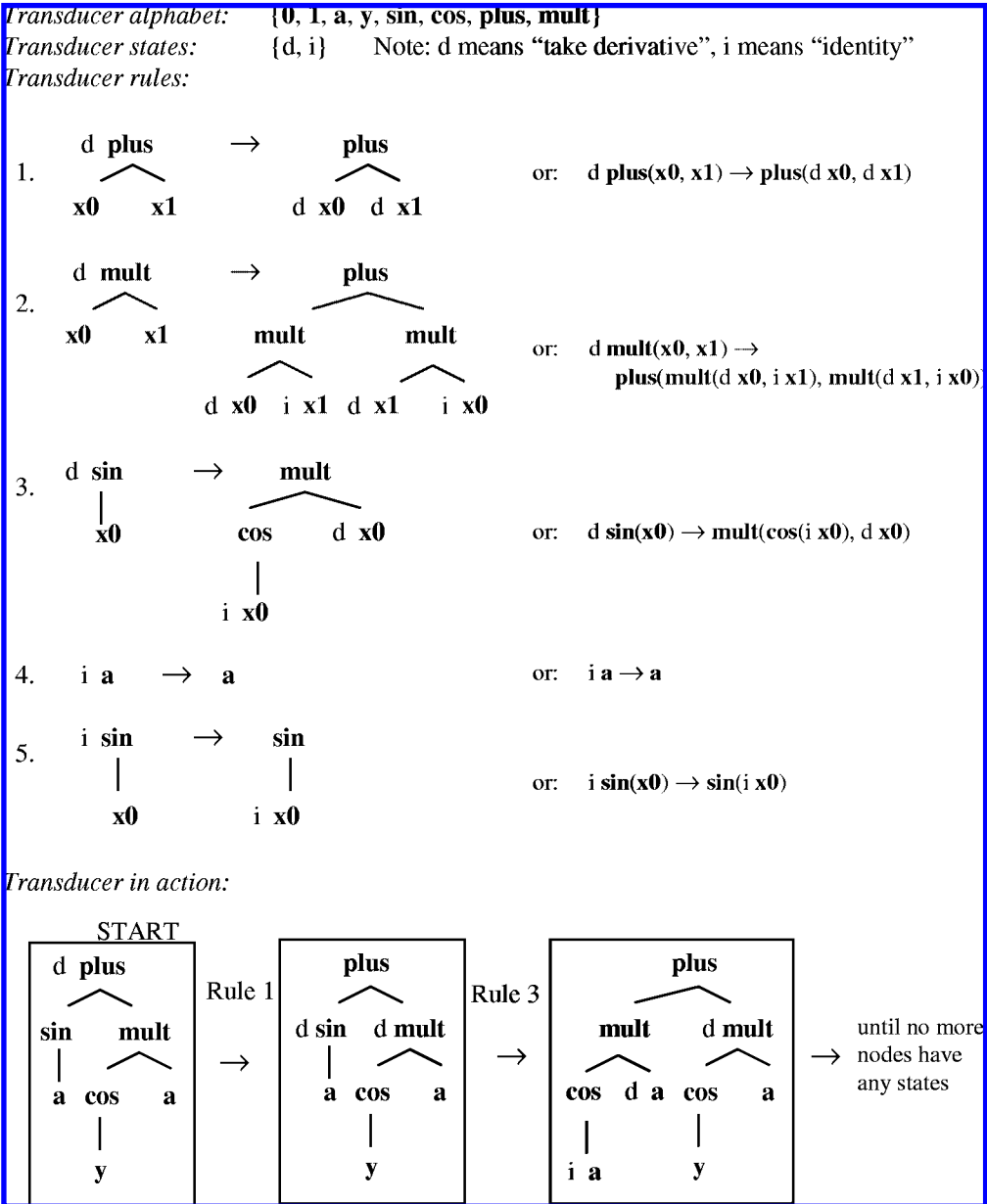
Figure 1 Part of a sample T tree transducer, adapted from Rounds (1970).
