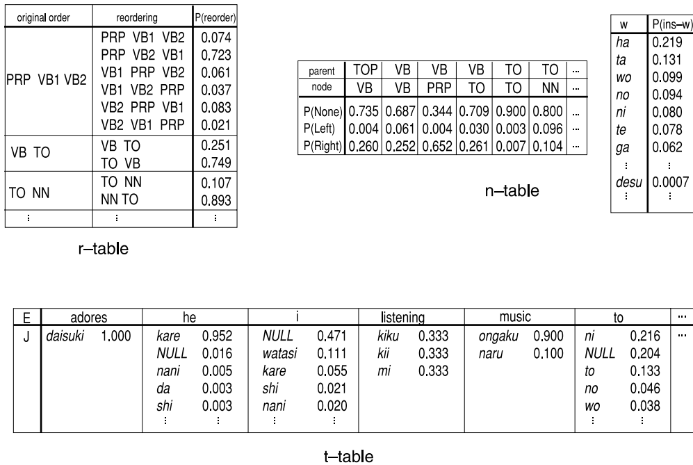
Figure 8 The parameter tables of Yamada and Knight (2001).
