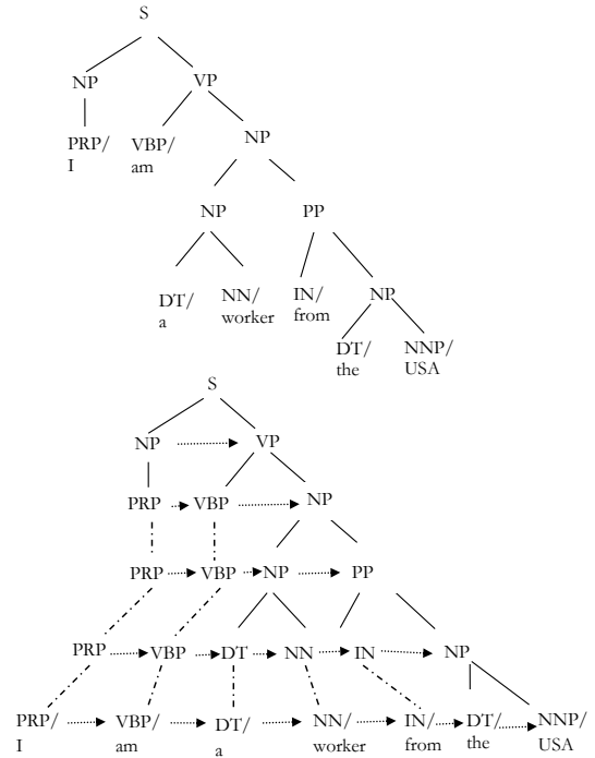
Figure 1: A regular constituent parse tree and its Expanded constituent tree.
