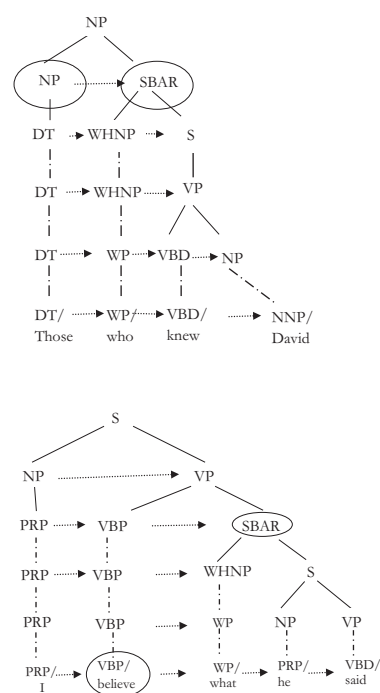
Figure 2: Expanded constituent parse tree for examples.
