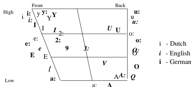
Figure 1: Vowel phonemes in Dutch, English, and German
