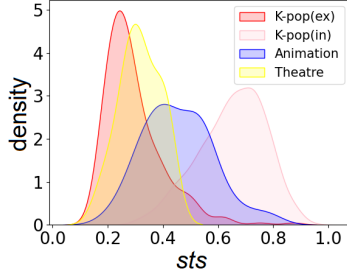
Figure 3: Density plots showing the distribution of line-by-line semantic textual similarity ( sts ) between the English and Korean lyrics for K-pop songs, considering both instances where untranslated English lyrics are included and where they are excluded, animated musical songs, and theatre songs.
