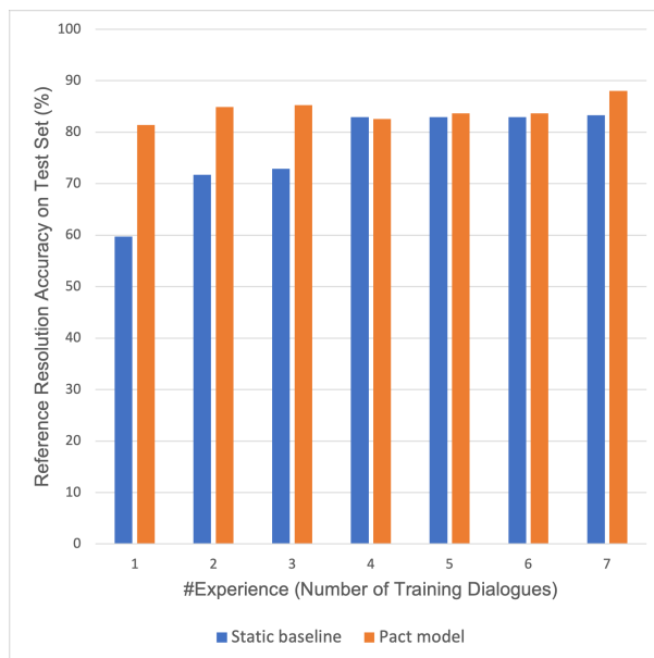
Figure 5: Reference resolution accuracy showing faster convergence of the Pact Model with limited experience compared to the static baseline.
