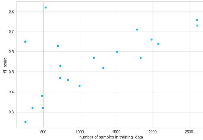
Figure 4: Error Analysis: Label Frequency in training data vs f1-performance of the system.
