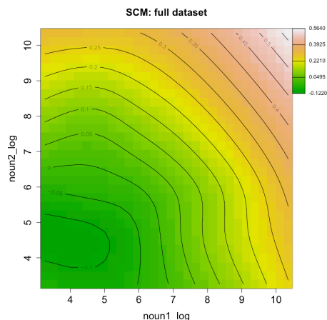
Figure 2: 2-way interaction and frequency effects in full dataset: the more frequent two nouns are, the more likely they are to share classifiers.
