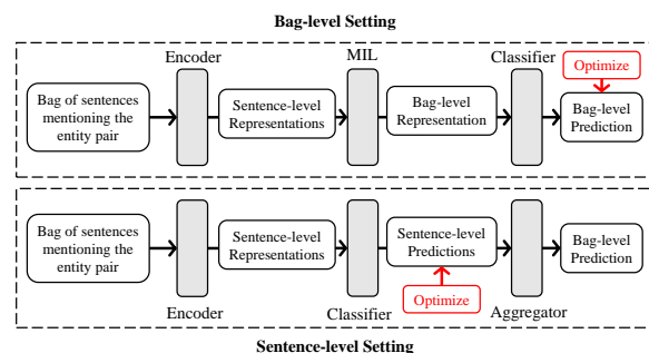
Figure 1: The bag-level and sentence-level pipelines of DSRE.
