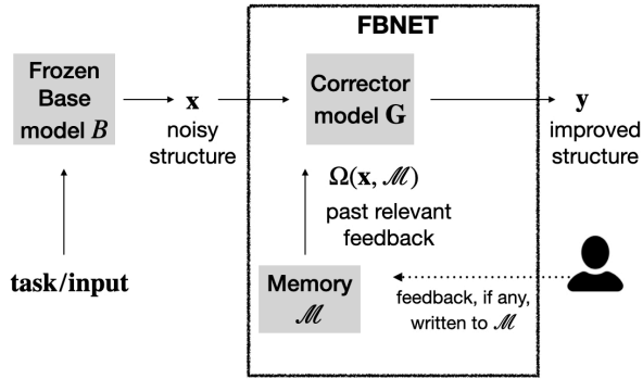
Figure 2: Proposed architecture: (left) \mathbf{B} does not account for user feedback. (right) FBNET maintains a memory \mathcal{M} of corrective feedback, and searches for feedback from prior queries with similar error intent as \mathbf{x} using a retrieval function \Omega . \mathbf{x} is then concatenated to the retrieved feedback to form the input to the corrector model \mathbf{G} . Users can also give new feedback which is added to \mathcal{M} . In this work, we focus on script generation models that might generate an erroneous script which are correctable using an edit (feedback).
