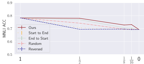
Figure 5: Comparison between different heads selection methods over MNL. Our method outperforms all other alternatives. The x-axis represents the fraction of input-dependent attention heads.
