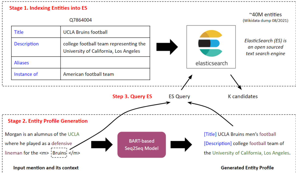
Figure 2: Candidate retrieval based on entity profiling.
