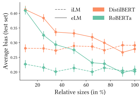
Figure 2: Bias removal. The x-axis represents the relative size ( x = \frac{1-p}{p} in percentages) between the modified environment and the unmodified one and the y-axis is the average bias for both iLM and eLM. Note that, according to Pairformance, \mathbb{P}(iLM \text{ beats } eLM) > 0.95 when the relative size is < 80\% , and that eLM and iLM become indistinguishable for relative sizes > 80\% . Due to space, we report the results obtained by ensLM and mtLM in Appendix B.2 which also shows that they perform in between iLM and eLM.
