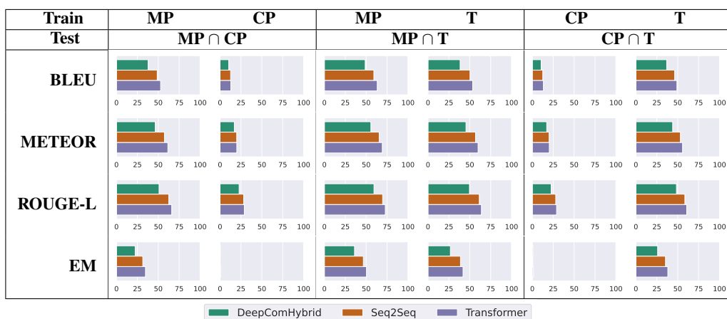
Figure 7: Results of comment generation models with filtering near-duplicates using the same_code configuration, on TestC sets.
