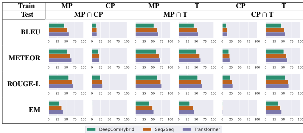
Figure 13: Results of comment generation models on common test sets.
