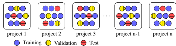
Figure 2: Mixed-project methodology.
