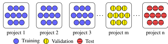
Figure 3: Cross-project methodology.
