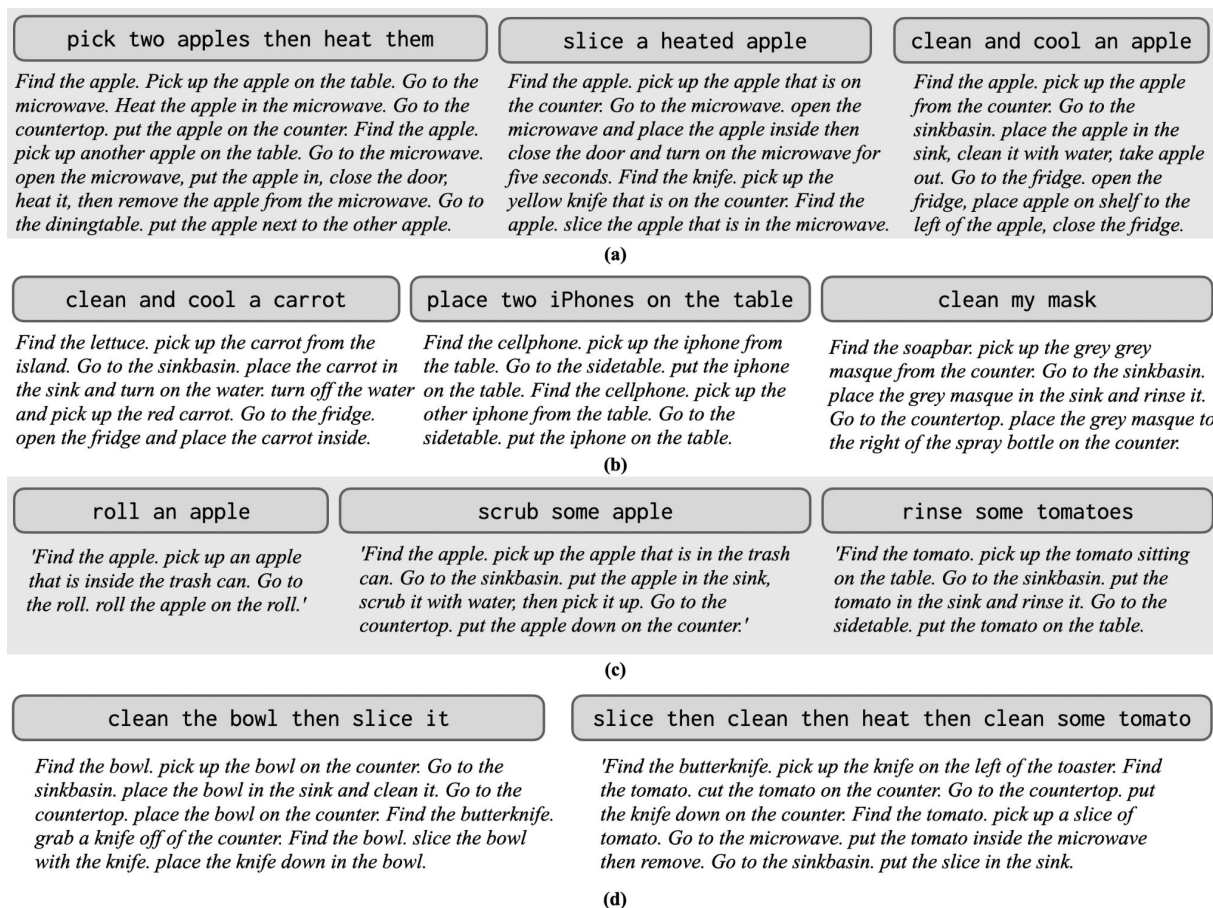
Figure 5: Successes and failures of \pi^C in out-of-distribution (OOD) settings including novel (a) sub-task orders (b) objects (c) verbs. The use of a pretrained LM as the backbone of the planning model means that models produce correct or plausible plans for many of these out-of-distribution goals. (d) Other failure modes: The model fails to predict actions based on the true affordances of objects and cannot generate arbitrarily long plans.
