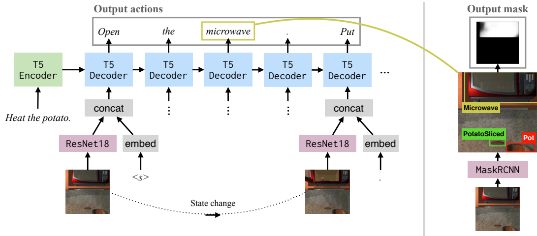
Figure 6: Model architecture for \pi^E , seq2seq and seq2seq2seq: Language parametrized sub-task/goal is input to the encoder and actions templated in natural language are generated sequentially token-wise. The predictions made are conditioned on the visual field of view of the agent at every time step along with the token generated the previous time step. At the end of every low-level action (when '.' is generated) the action the executed. For manipulation actions, the mask corresponding to the the object predicted is selected from the predictions of a MaskRCNN model on the visual state. Navigation actions do not operate over objects. Once the action is taken, the environment returns the updated visual state and the policy continues to be unrolled until termination (STOP).
