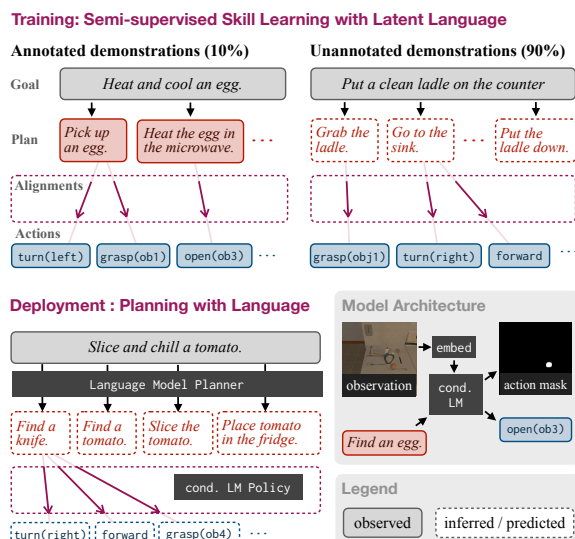
Figure 1: Hierarchical imitation learning using weak natural language supervision. During training, a small number of seed annotations are used to automatically segment and label unannotated training demonstrations with natural language descriptions of their high-level structure. When deployed on new tasks, learned policies first generate sequences of natural language subtask descriptions, then modularly translate each description to a sequence of low-level actions.
