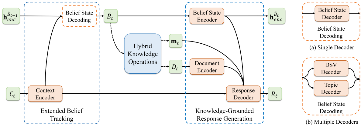
Figure 2: Overview of HyKnow. Solid arrows denote the input/output of the encoders or decoders. Dashed arrows denote the knowledge operations. C_t , \mathbf{m}_t , D_t and R_t represent turn t 's dialog context, DB query result, relevant document and system response. \tilde{B}_t and \mathbf{h}_{enc}^{\tilde{B}_t} denote the extended belief state and its hidden states at turn t . The decoding of \tilde{B}_t (orange dashed box) is implemented in two different ways: (a) using a single decoder to generate the whole state, and (b) using two decoders to generate the domain-slot-value (DSV) triples and the topic separately.
