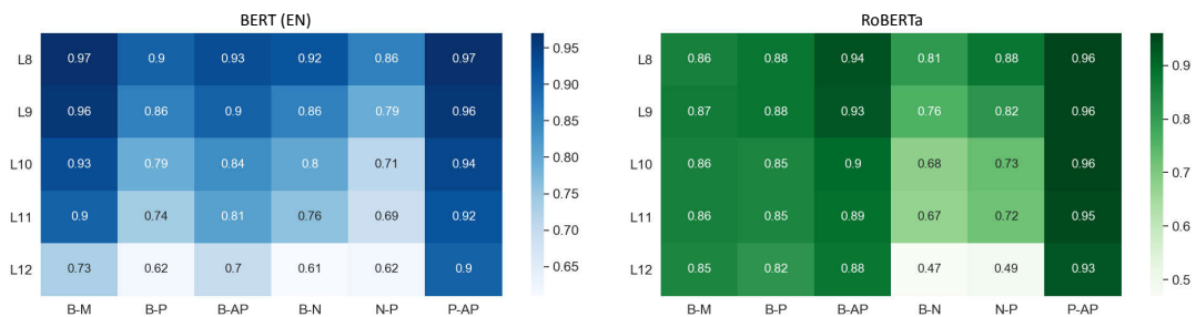
Figure 3: Topological similarity (l-CKA) for pairs of BERT and RoBERTa variants, before and after different fine-tuning steps (B, M, P, AP, and N). Rows: transformer layers; Columns: pairs of transformer variants in comparison.
