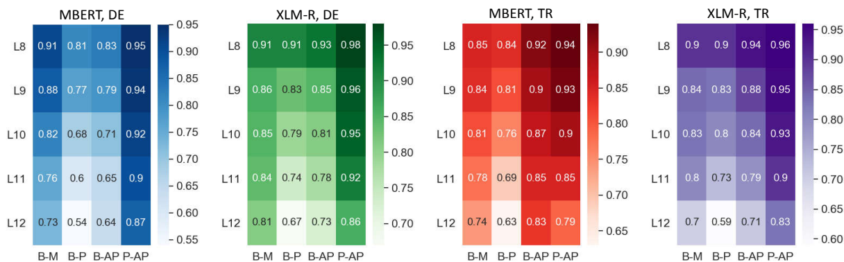
Figure 4: Analysis of topological similarity (l-CKA) for variants of mBERT and XLM-R before and after IPT and ILMT (B, M, P, AP) in zero-shot transfer experiments. Results shown for intermediate parsing on DE and TR data.
