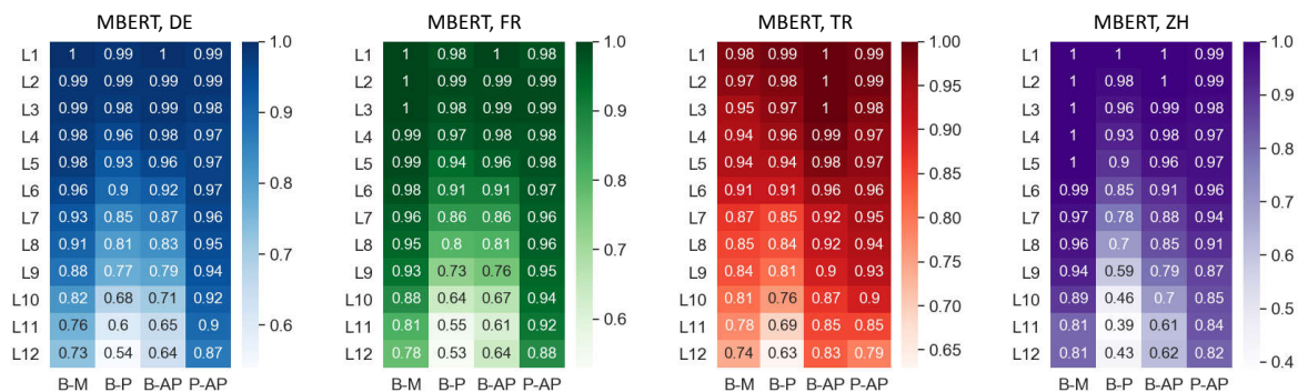
Figure 6: Full results of the topological similarity analysis (l-CKA) for variants of mBERT before and after IPT and ILMT (B, M, P, AP) for the following target languages (left to right): DE, FR, TR, and ZH.
