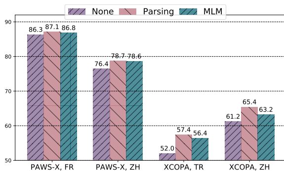
Figure 2: Comparison of IPT and ILMT in zero-shot language transfer experiments with mBERT on PAWS-X (FR and ZH) and XCOPA (TR and ZH). None : no intermediate training; Parsing : intermediate parsing training; MLM : intermediate masked LM training.
