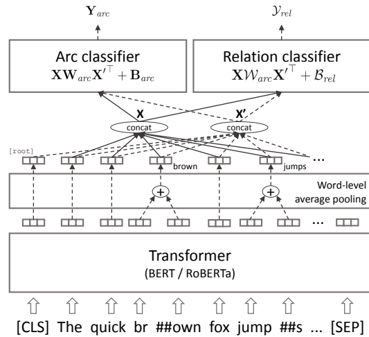
Figure 1: Architecture of our transformer-based biaffine dependency parser.
