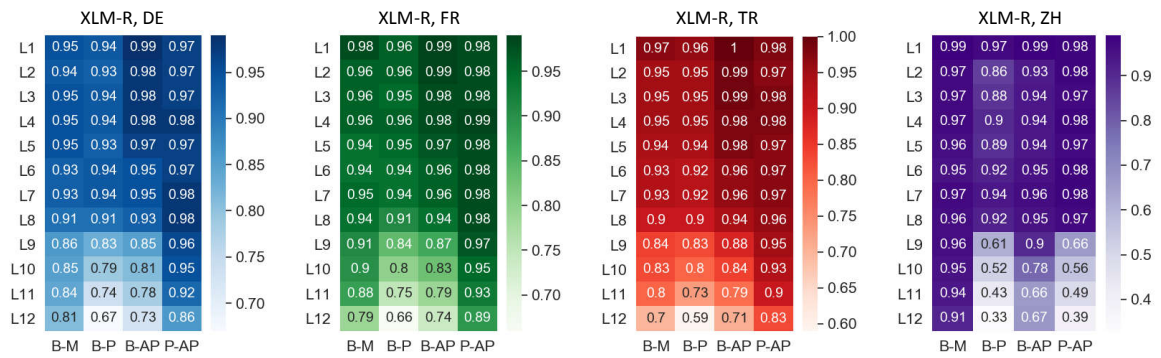
Figure 7: Full results of the topological similarity analysis (l-CKA) for variants of XLM-R before and after IPT and ILMT (B, M, P, AP) for the following target languages (left to right): DE, FR, TR, and ZH.
