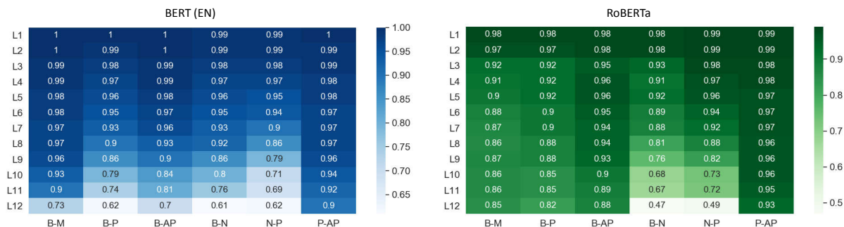
Figure 5: Full results of the topological similarity analysis (l-CKA) for pairs of BERT and RoBERTa variants, before and after different fine-tuning steps (B, M, P, AP, and N). Rows : transformer layers; Columns : pairs of transformer variants in comparison.
