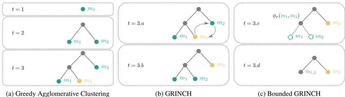
Figure 2: Bounded GRINCH . (a) Greedy agglomerative clustering produces a sub-optimal tree structure due to the order points are received. (b) The GRINCH (Monath et al., 2019) algorithm recovers from this mistake by reconfiguring the tree structure (in this case using a rotation operation). (c) To ensure the memory used by GRINCH remains bounded, we add a new operation— remove —that prunes two leaf nodes when the number of leaves exceeds a given size. Nodes are selected for removal using a scoring function \phi_r . In this case nodes m_1 and m_2 are selected, and their parent \tilde{m}_{1,2} becomes a new leaf.
